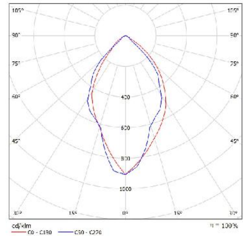
Light intensity distribution
