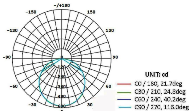
Luminous Intensity Curve
